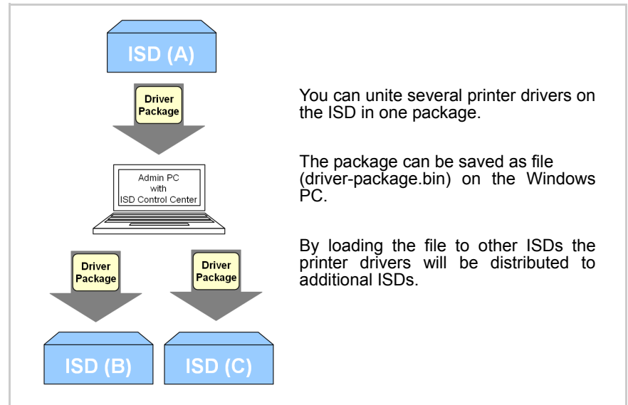
Fig. 9: Distribution of printer driver packages
