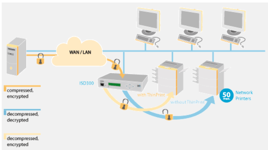
Fig. 20: ISD as ThinPrint® Gateway
