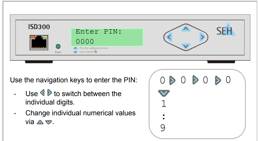
Fig. 13: ISD Device - Panel Lock
