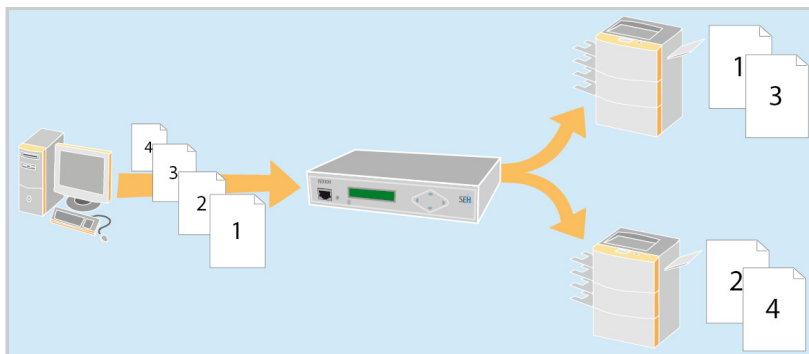
Fig. 11: Balance Queue
