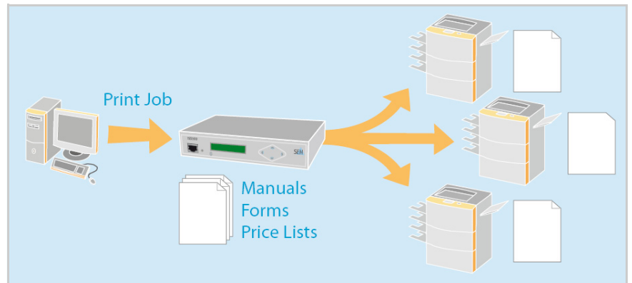
Fig. 12: Repository
