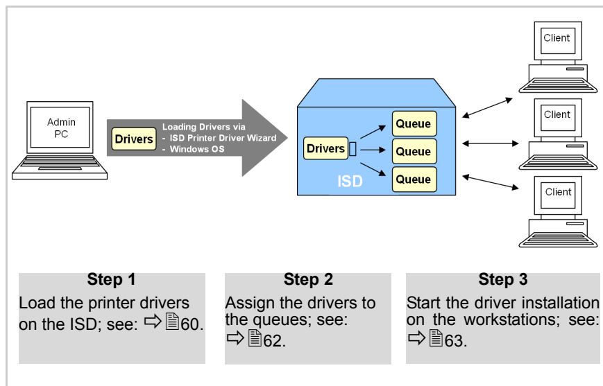
Fig. 8: Point and Print
