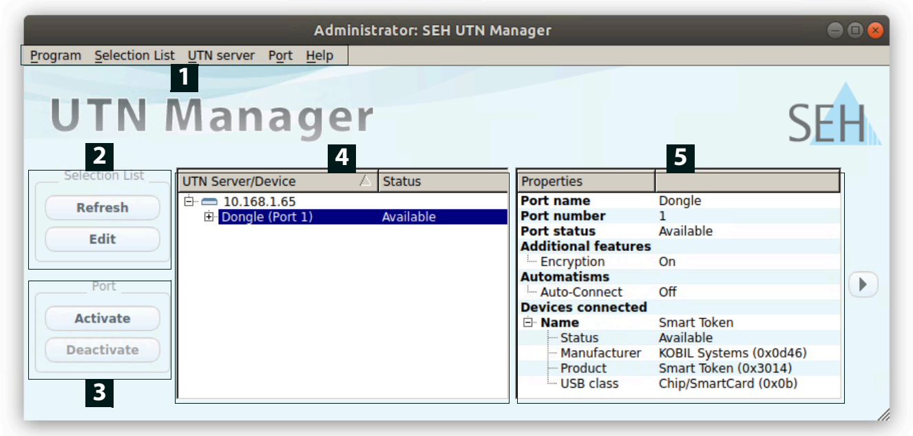
Figure 2.2-1: SEH UTN Manager
