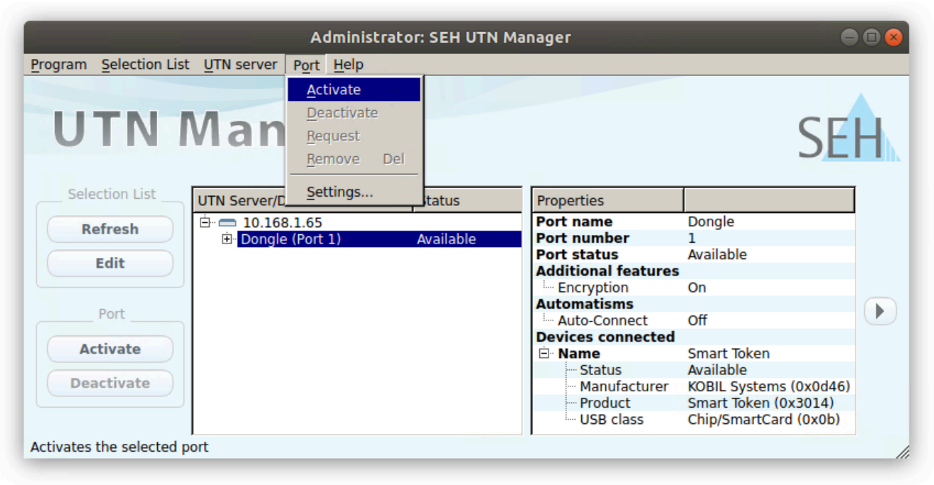
Figure 5.2-1: SEH UTN Manager – USB port activation
