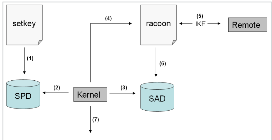
Fig. 9: IPsec procedure
